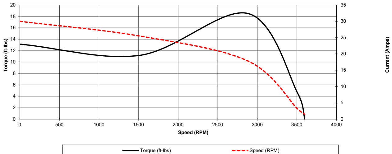
440T, 480T Dual Voltage DOL 3-Phase WYE Connection
